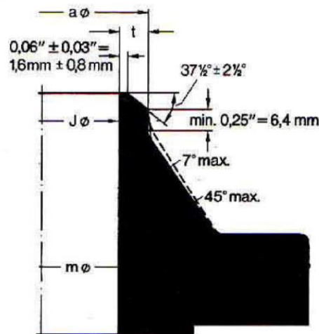
Bevel for Wall Thicknesses (t) 0,19" to 0,88" inclusive
