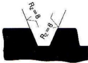
Ring Joint Facings
